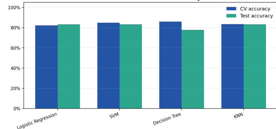
Classification model accuracy
